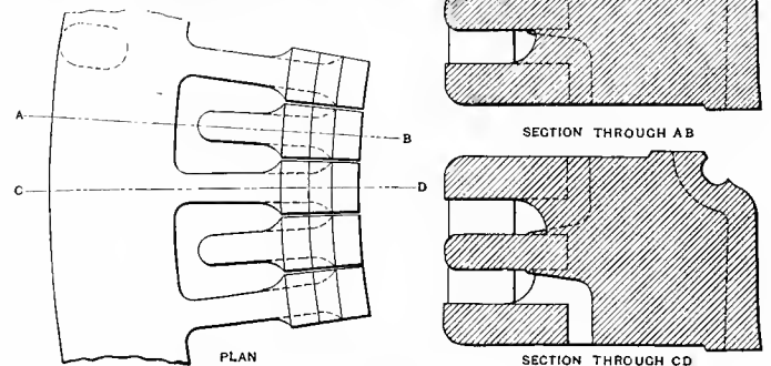
Figs. 5371-5373. Enlarged Plan and Cross Sections of Segmental Chilling-blocks.
